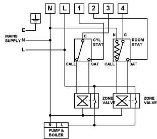
7. Fully Pumped System using RoomStat and CylinderStat and Two (2 Port) Motorised Valve with Auxiliary Switches
