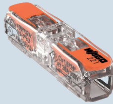
WAGO Inline 1-pole 0.2 - 4 mm 2 connector.
